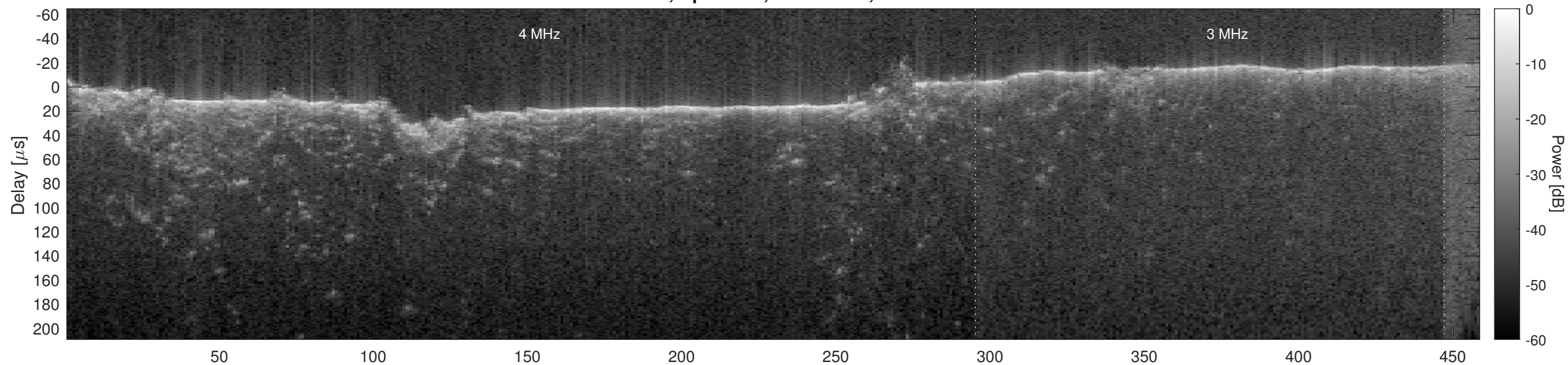
Orbit 2909, Optimized, No Window, Channel 2
