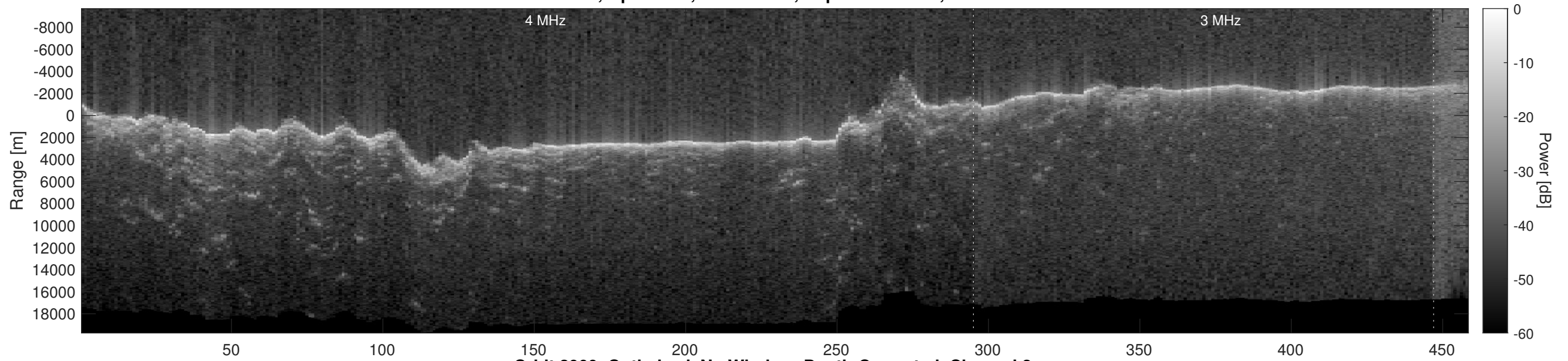
Orbit 2909, Optimized, No Window, Depth-Corrected, Channel 2
