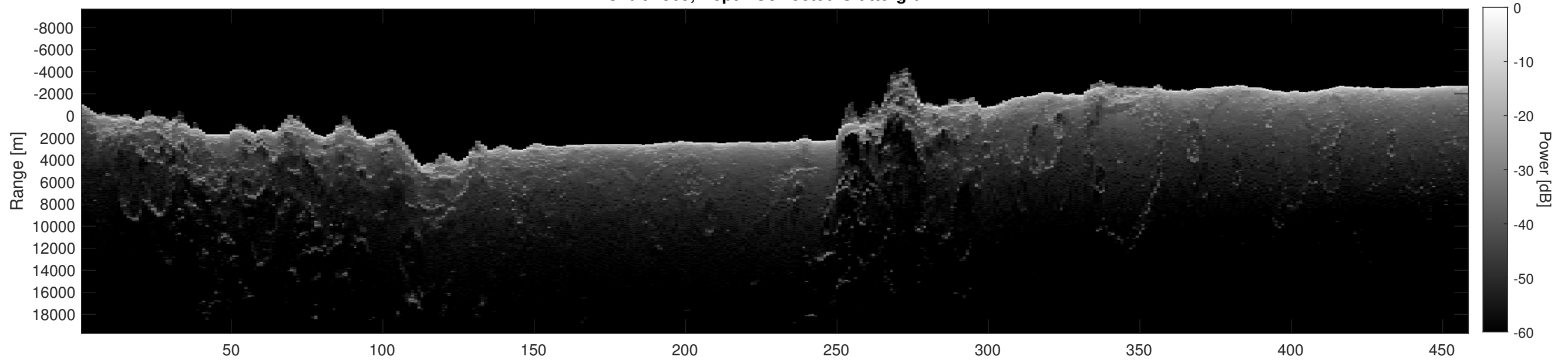
Orbit 2909, Depth-Corrected Cluttergram
