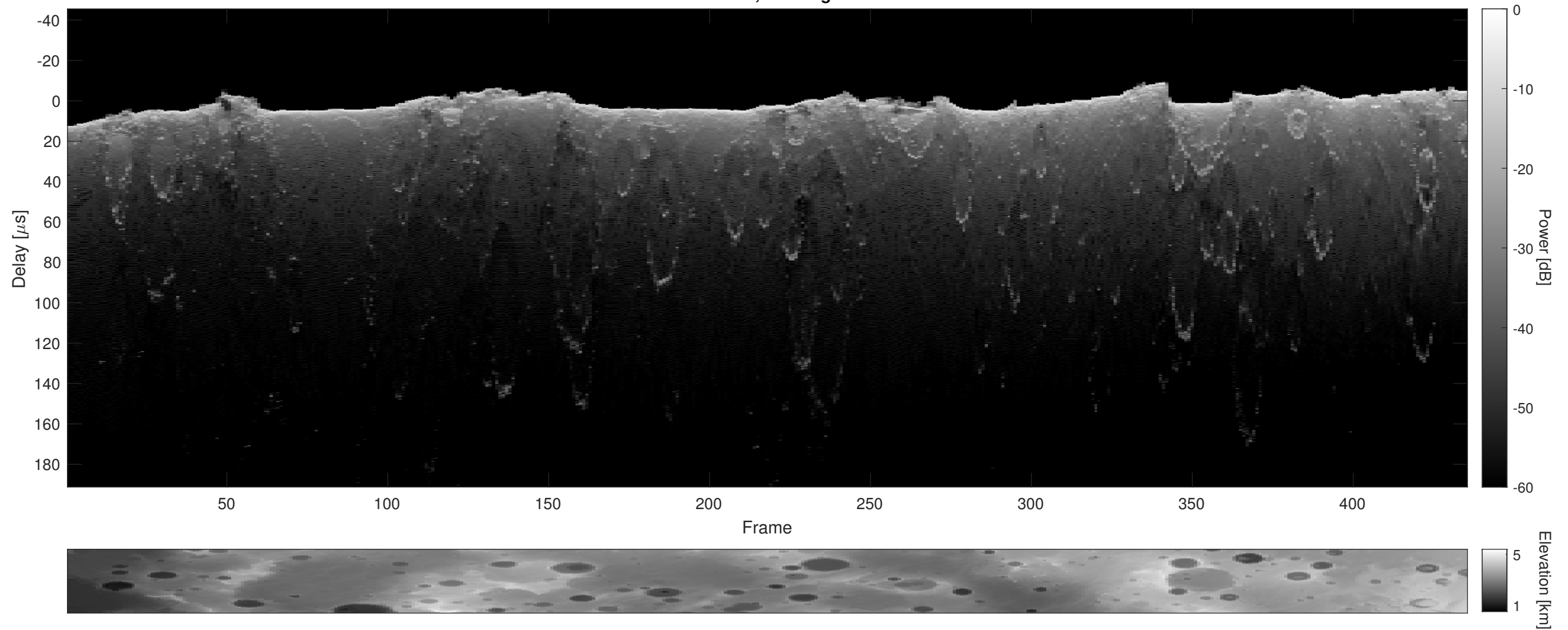
Orbit 2910, Cluttergram
