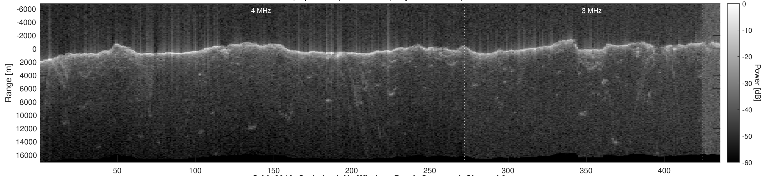
Orbit 2910, Optimized, No Window, Depth-Corrected, Channel 2
