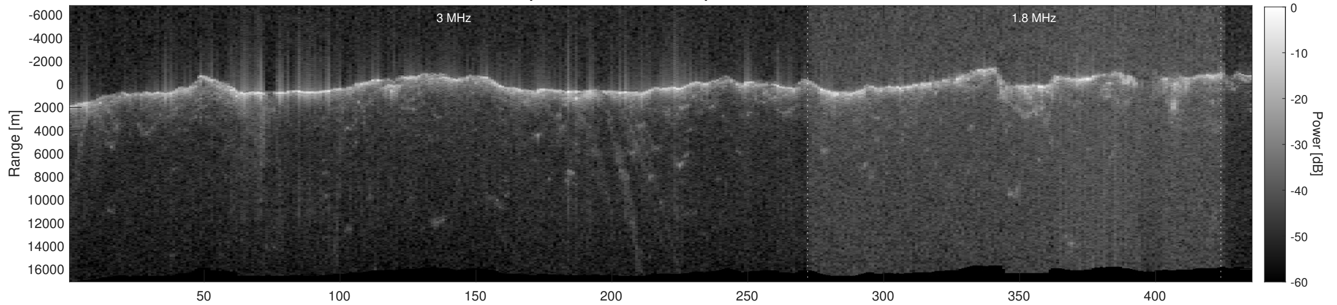
Orbit 2910, Depth-Corrected Cluttergram
