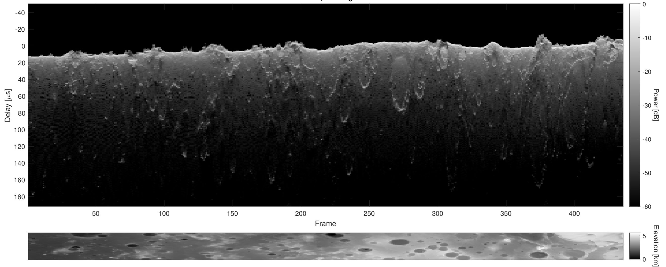
Orbit 2911, Cluttergram
