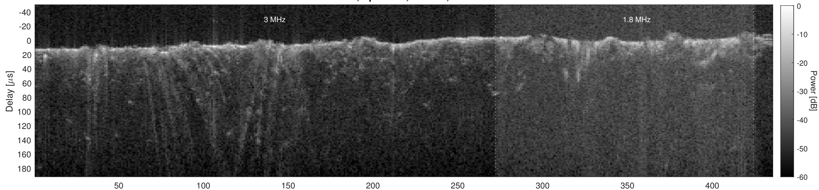
Orbit 2911, Cluttergram
