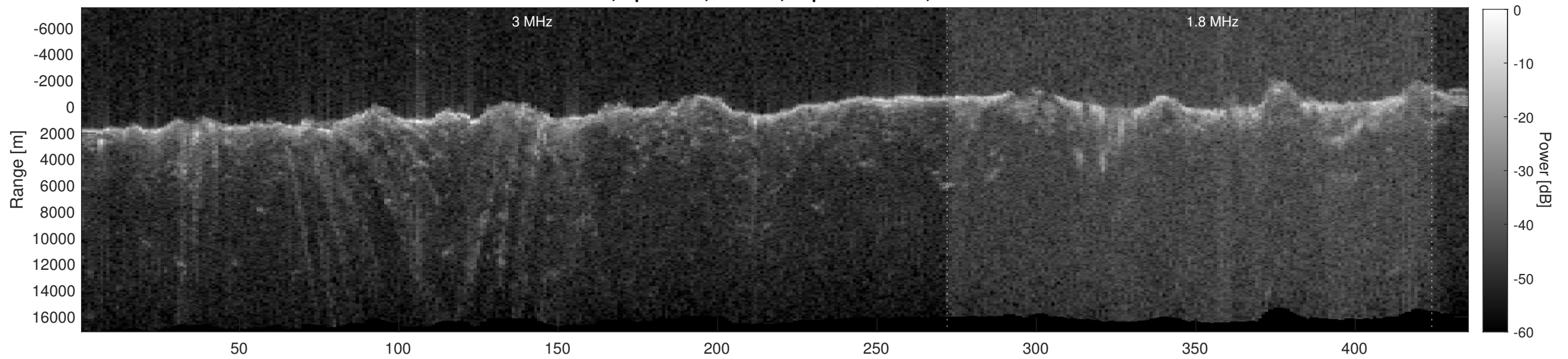
Orbit 2911, Depth-Corrected Cluttergram
