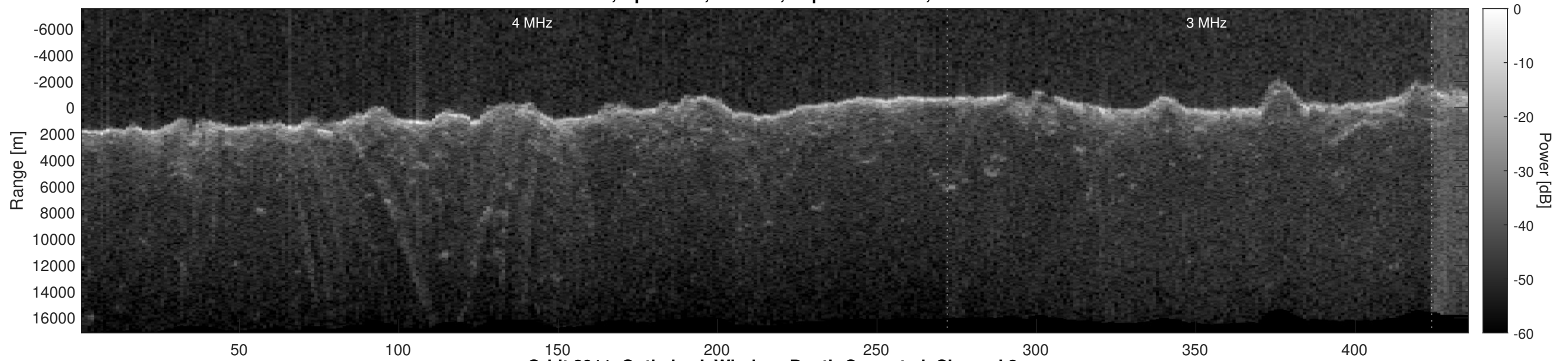
Orbit 2911, Optimized, Window, Depth-Corrected, Channel 2
