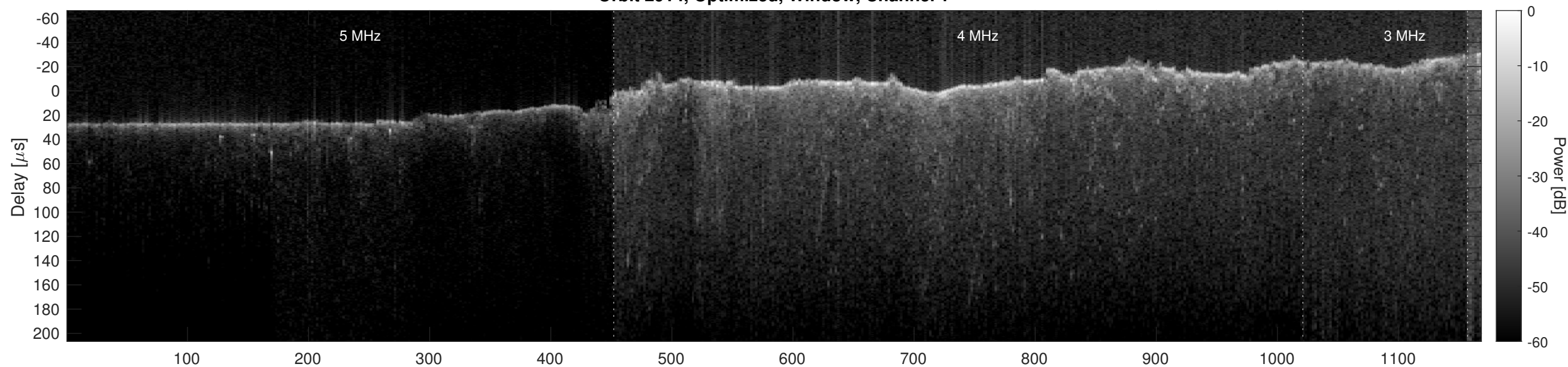
Orbit 2914, Optimized, Window, Channel 2
