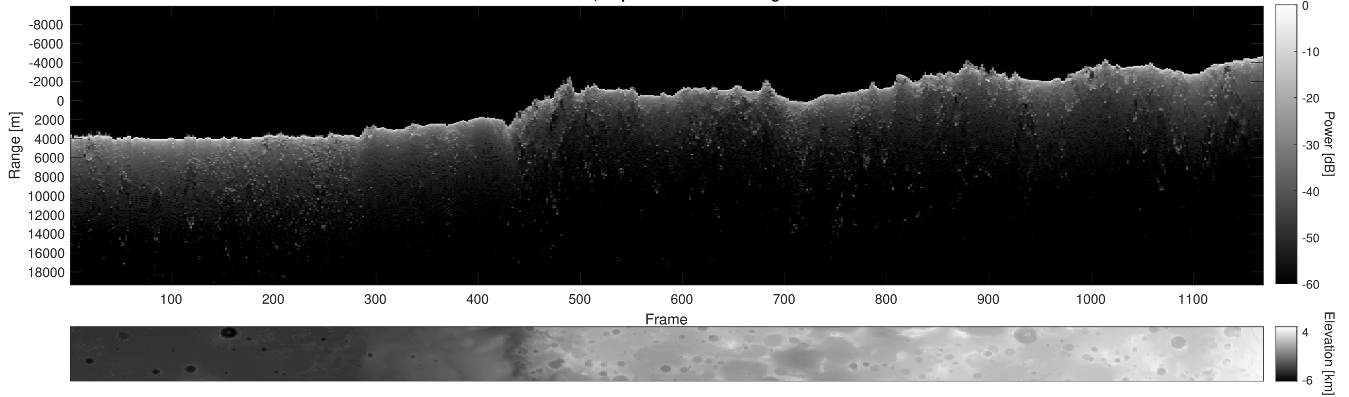
Orbit 2914, Depth-Corrected Cluttergram
