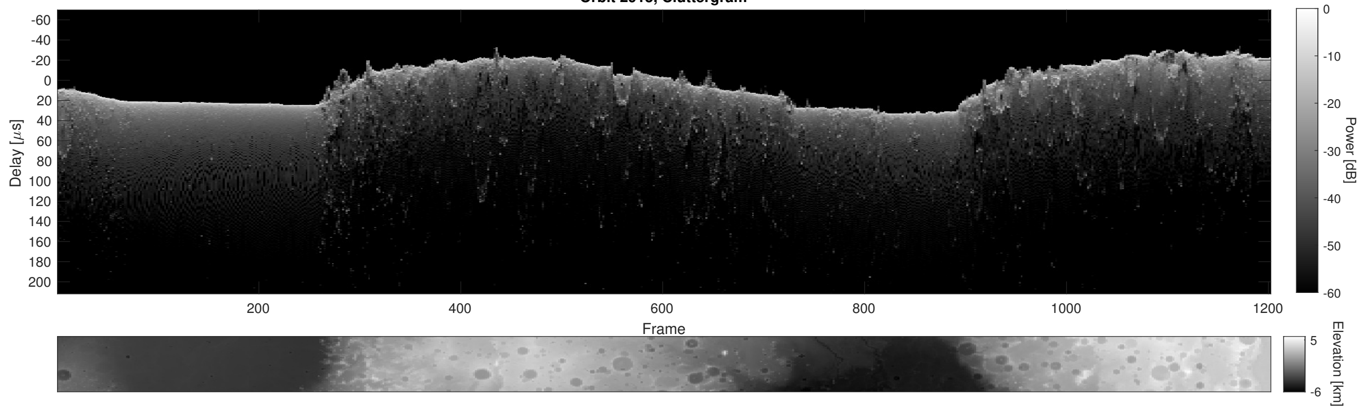
Orbit 2915, Cluttergram
