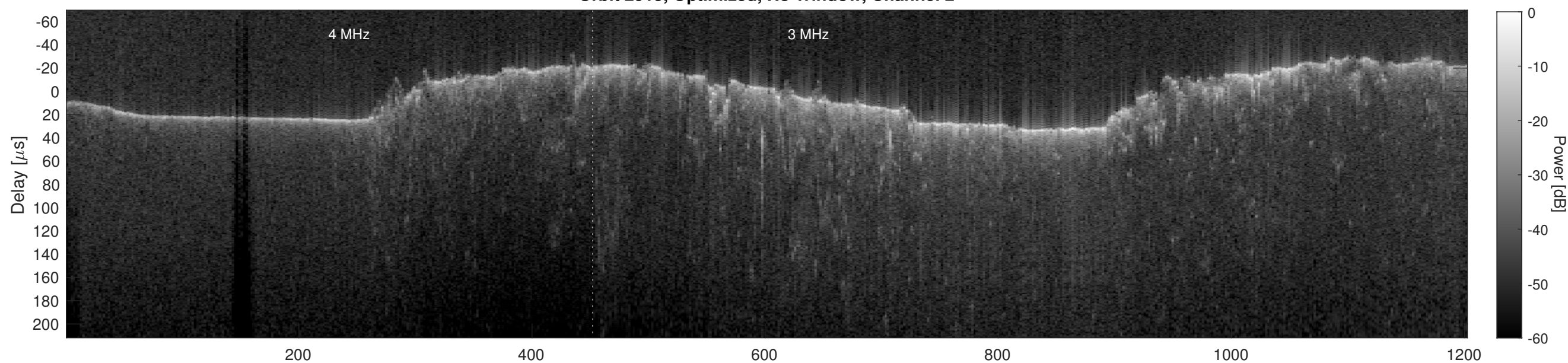
Orbit 2915, Cluttergram
