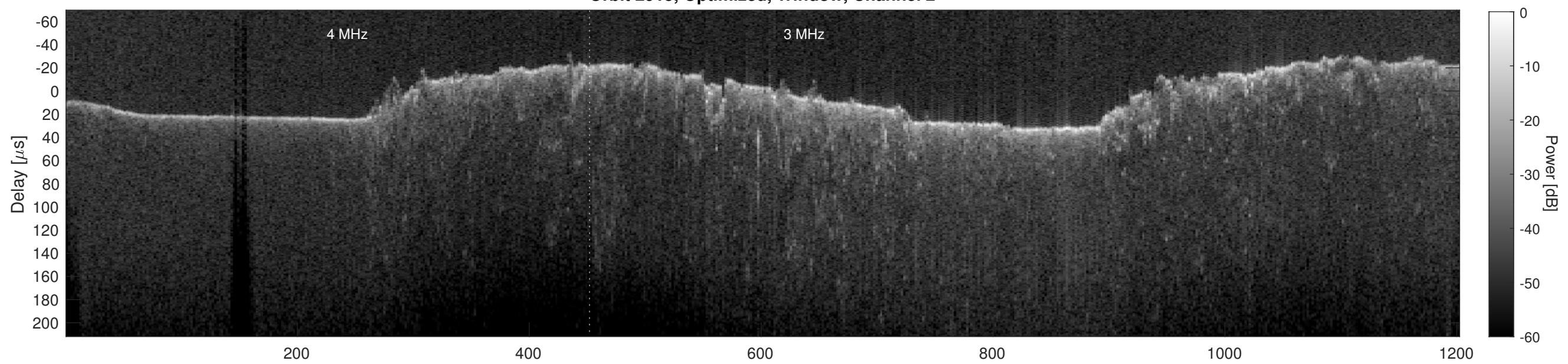
Orbit 2915, Cluttergram
