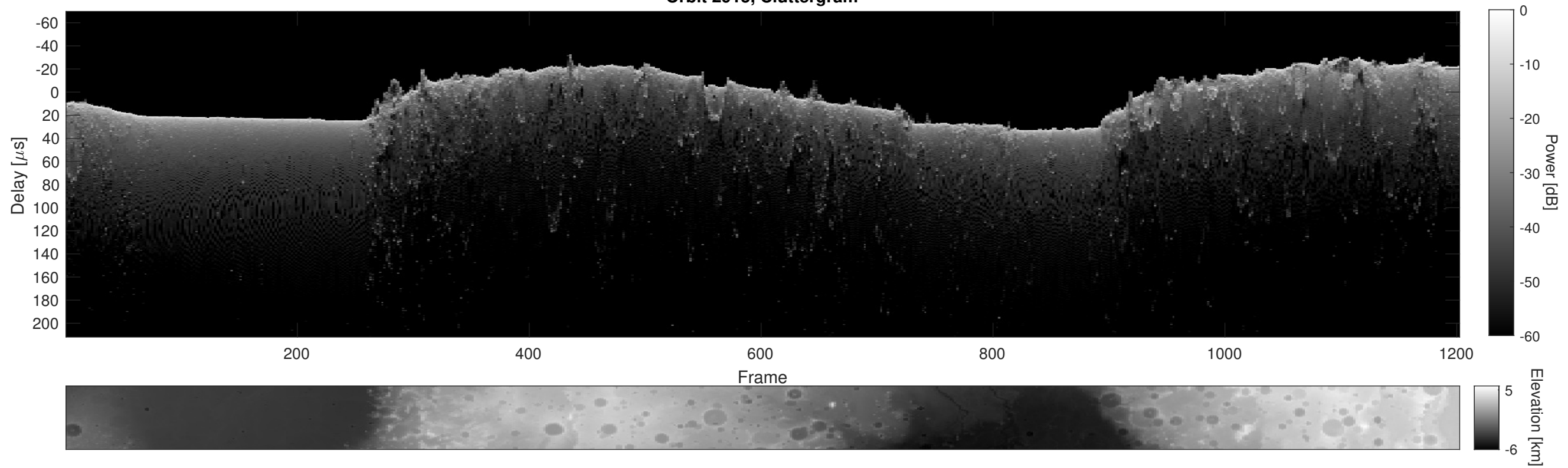
Orbit 2915, Cluttergram
