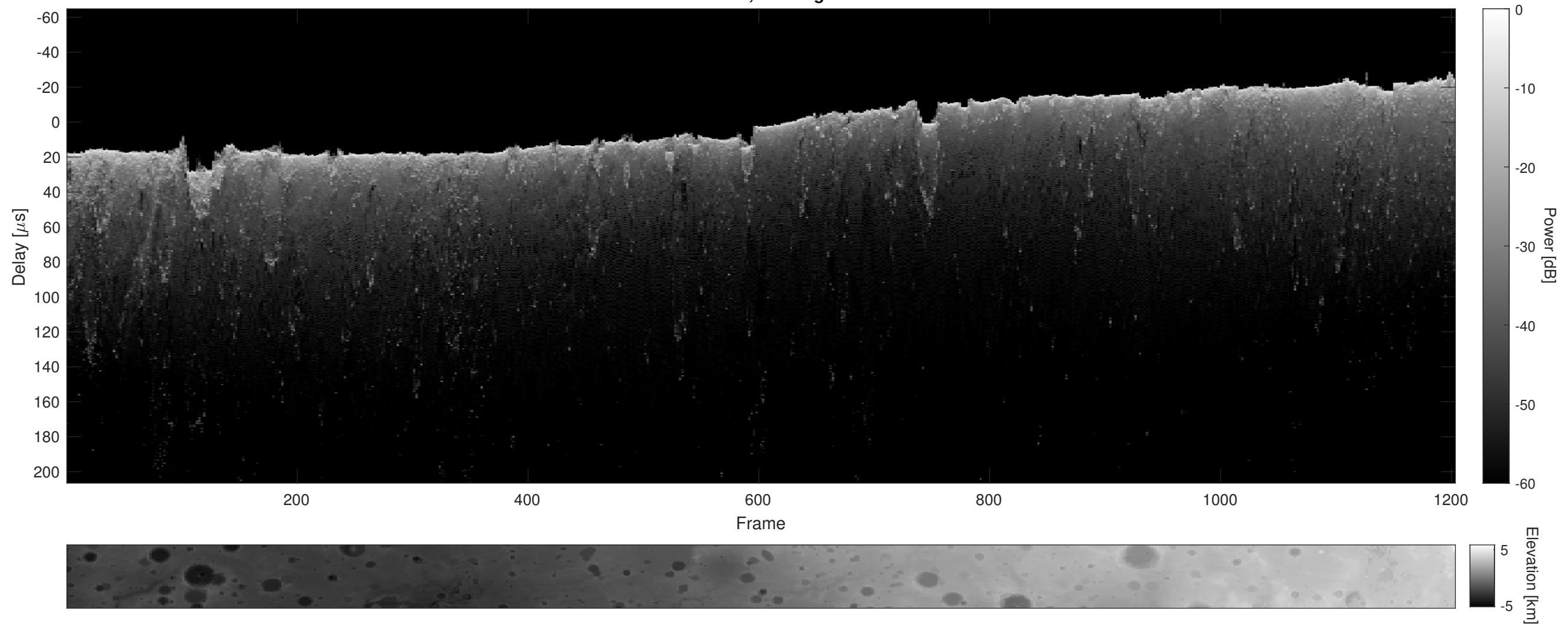
Orbit 2916, Cluttergram
