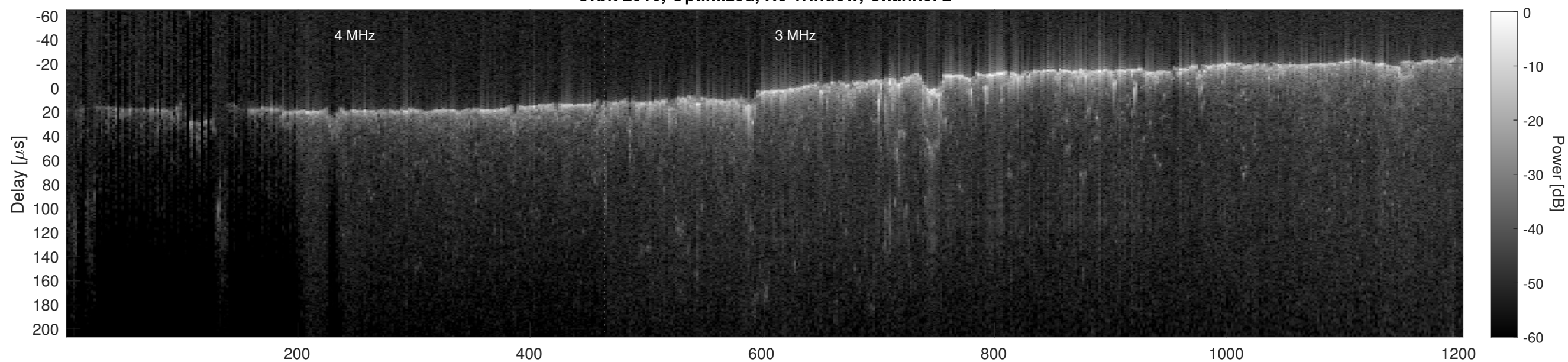
Orbit 2916, Cluttergram
