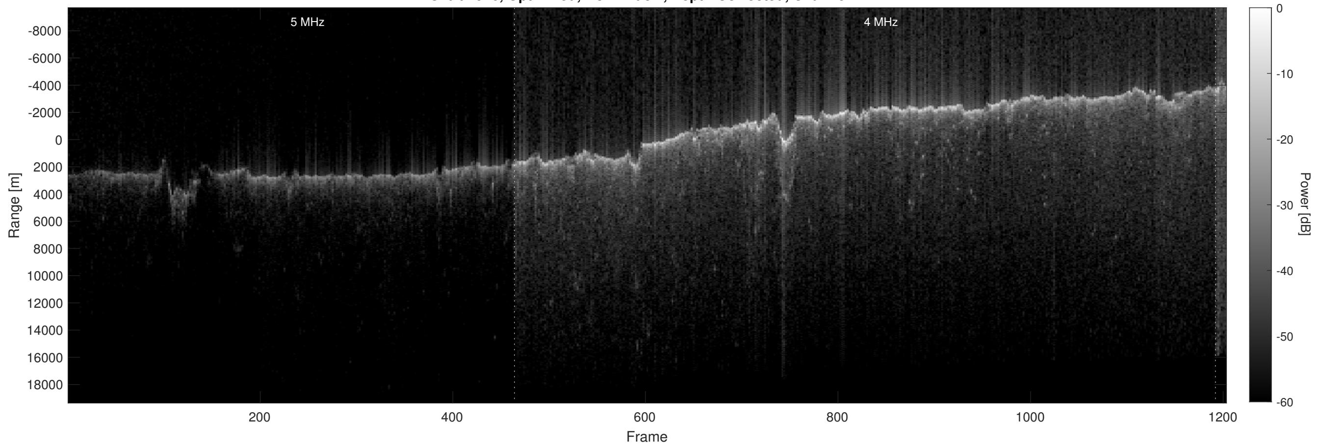
Orbit 2916, Optimized, No Window, Depth-Corrected, Channel 2
