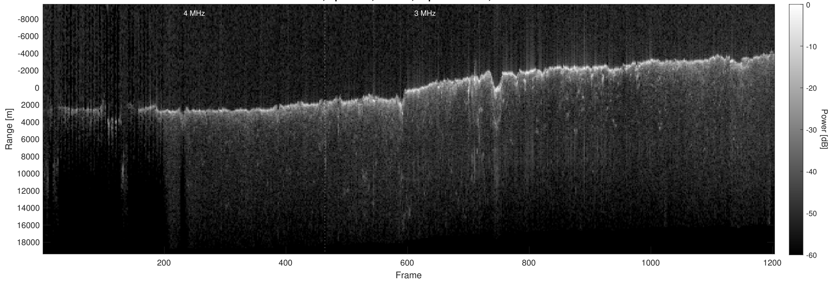
Orbit 2916, Optimized, Window, Depth-Corrected, Channel 2
