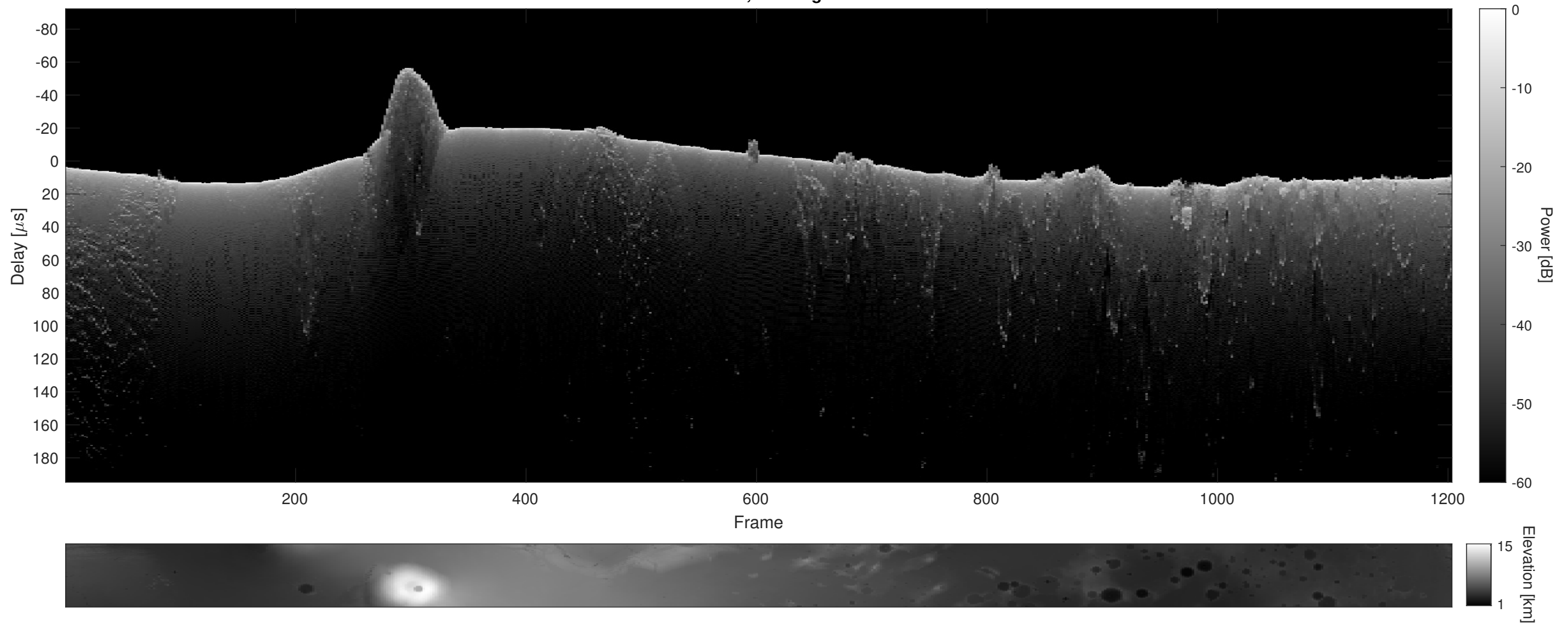
Orbit 2917, Cluttergram
