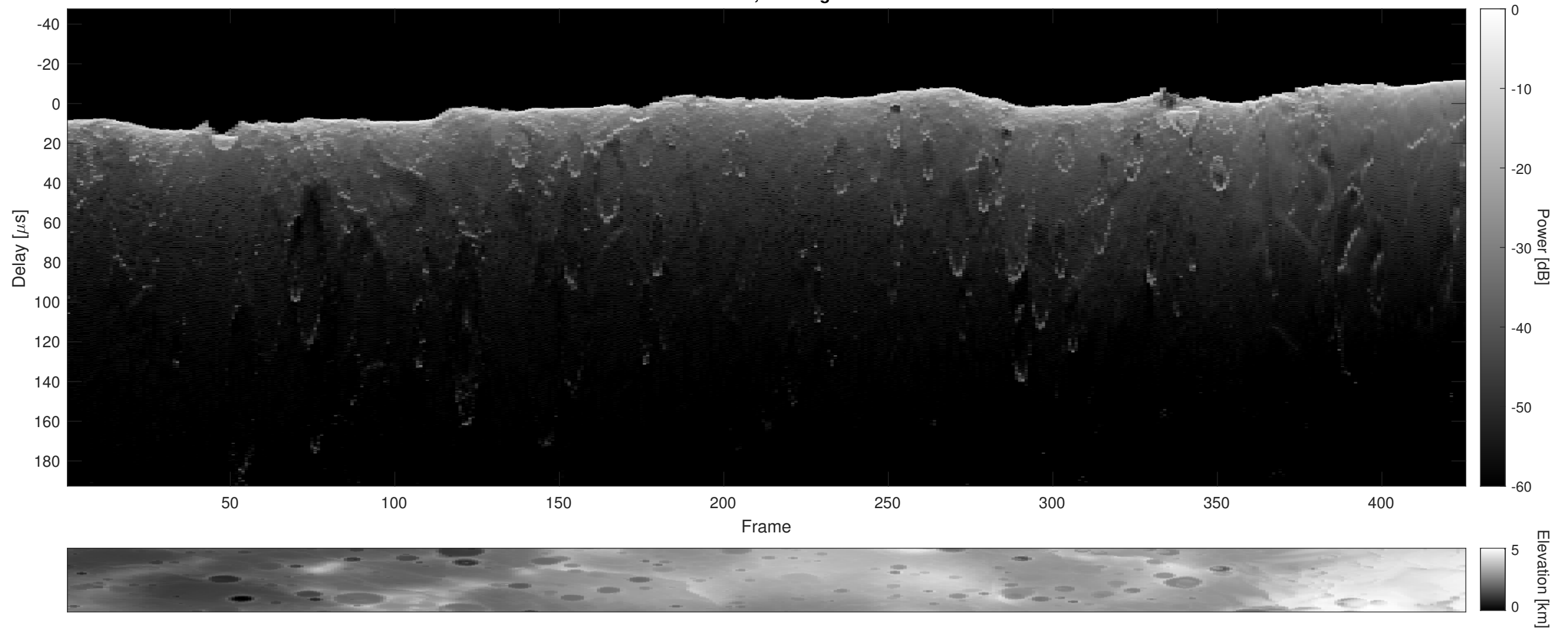
Orbit 2918, Cluttergram
