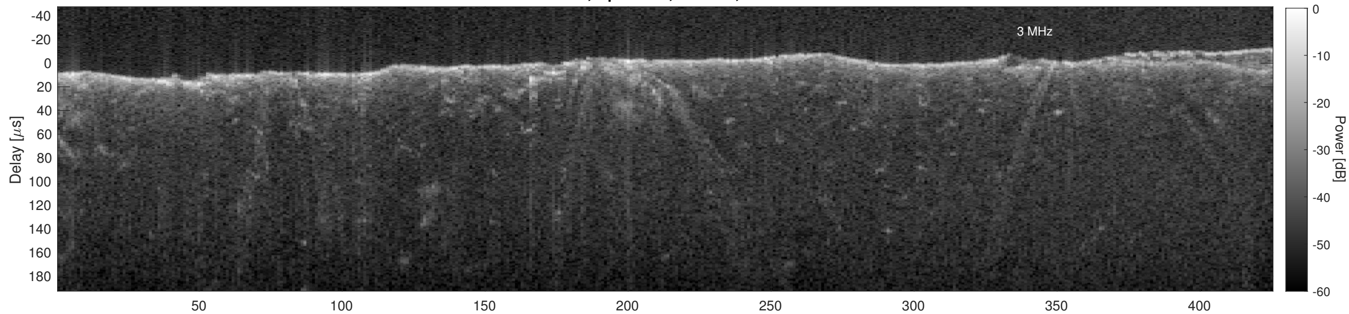
Orbit 2918, Cluttergram
