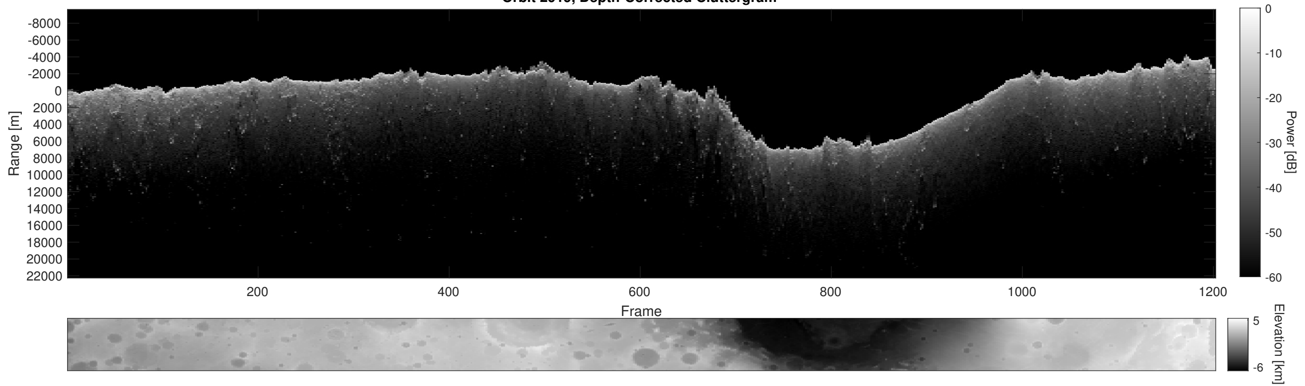
Orbit 2919, Depth-Corrected Cluttergram
