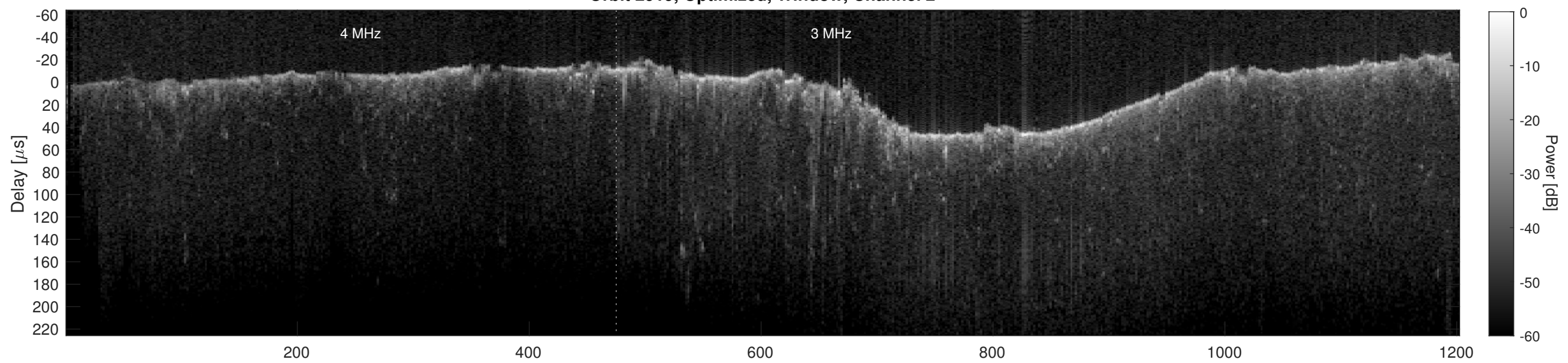
Orbit 2919, Cluttergram
