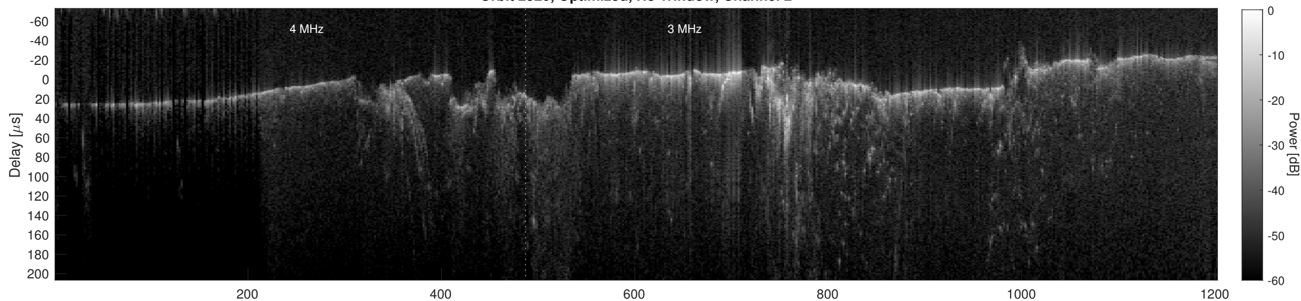
Orbit 2920, Cluttergram
