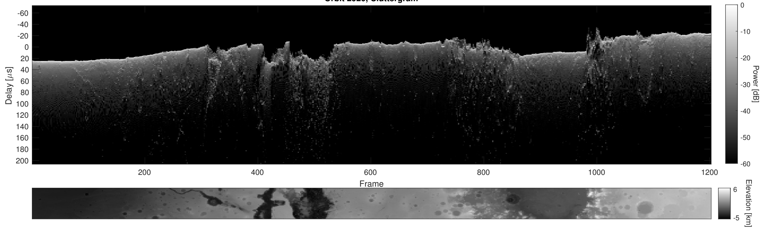
Orbit 2920, Cluttergram
