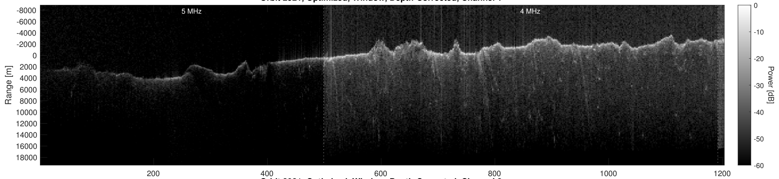
Orbit 2921, Optimized, Window, Depth-Corrected, Channel 2
