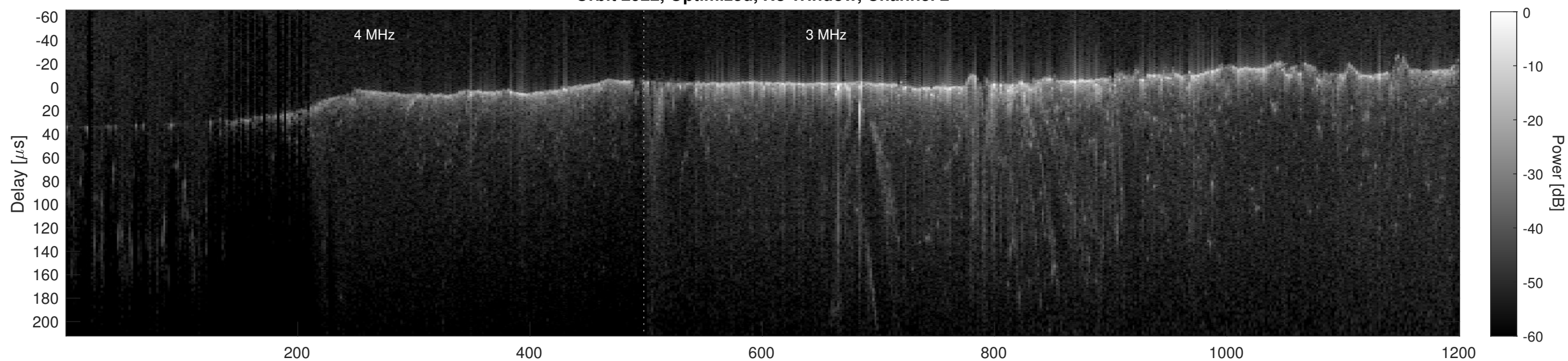
Orbit 2922, Cluttergram
