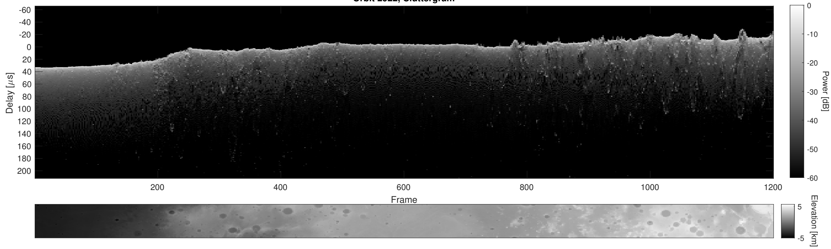
Orbit 2922, Cluttergram
