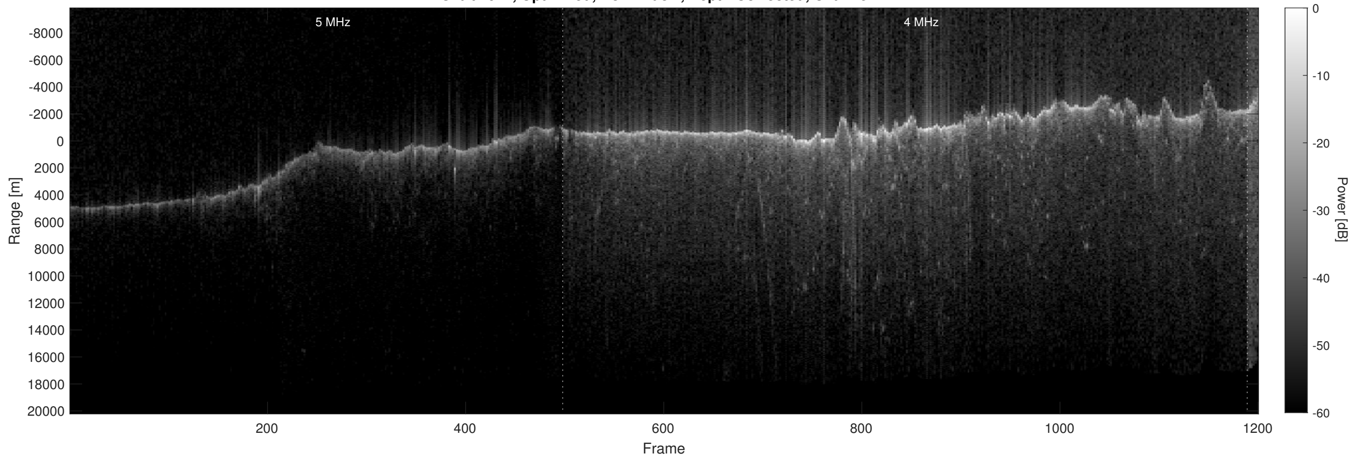
Orbit 2922, Optimized, No Window, Depth-Corrected, Channel 2
