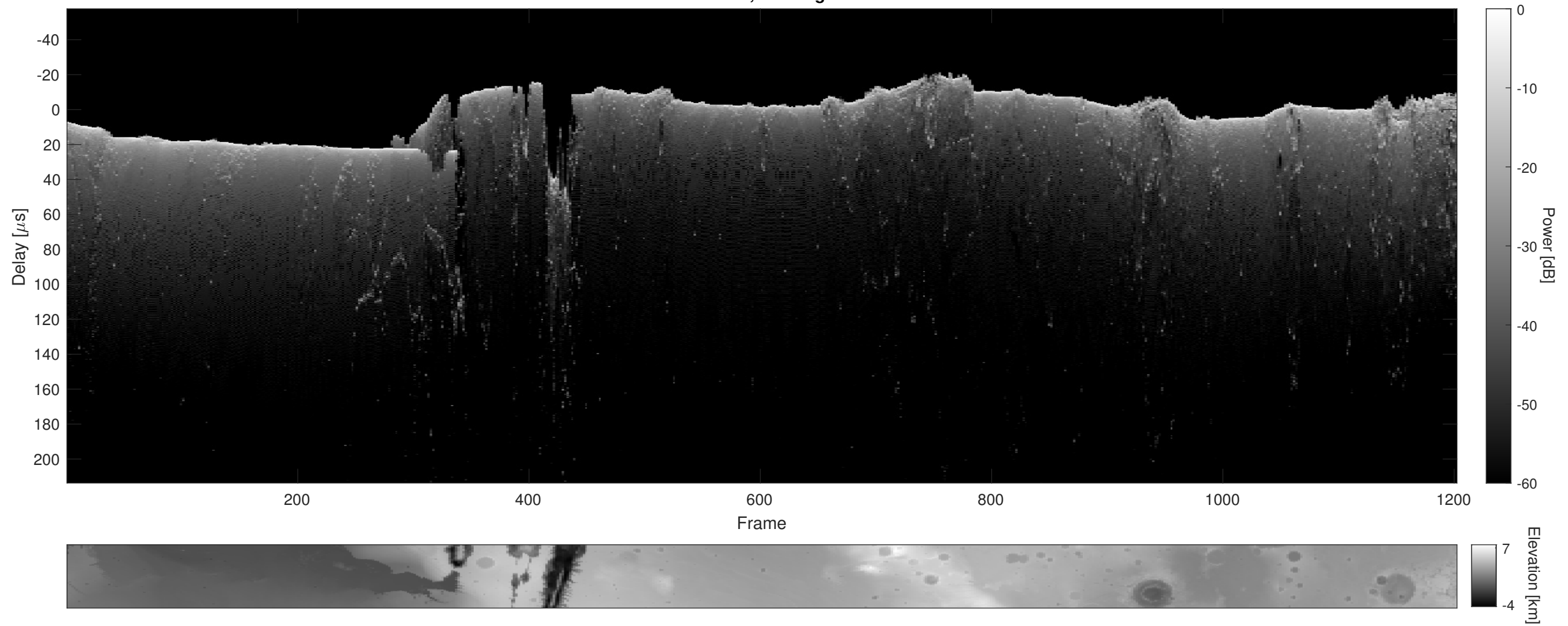
Orbit 2924, Cluttergram
