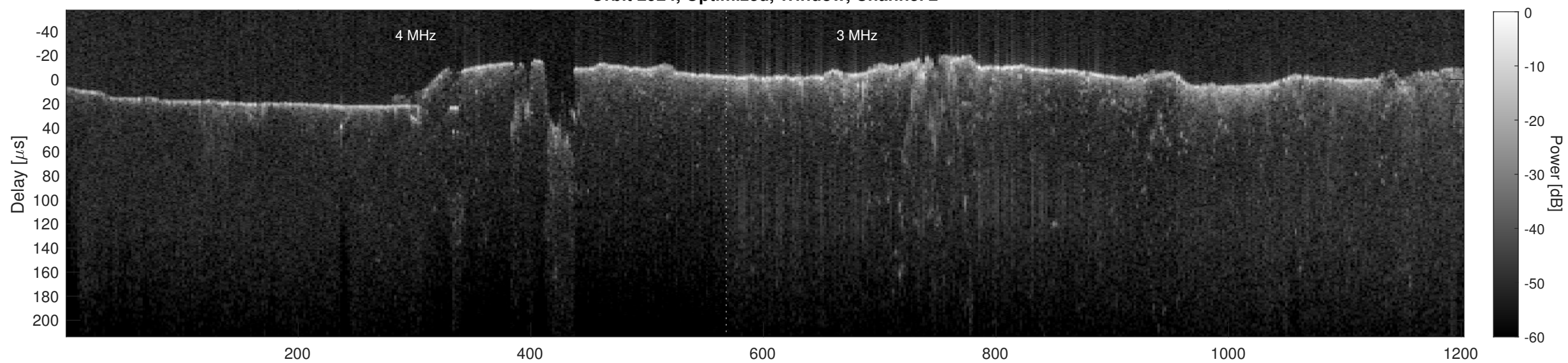
Orbit 2924, Cluttergram
