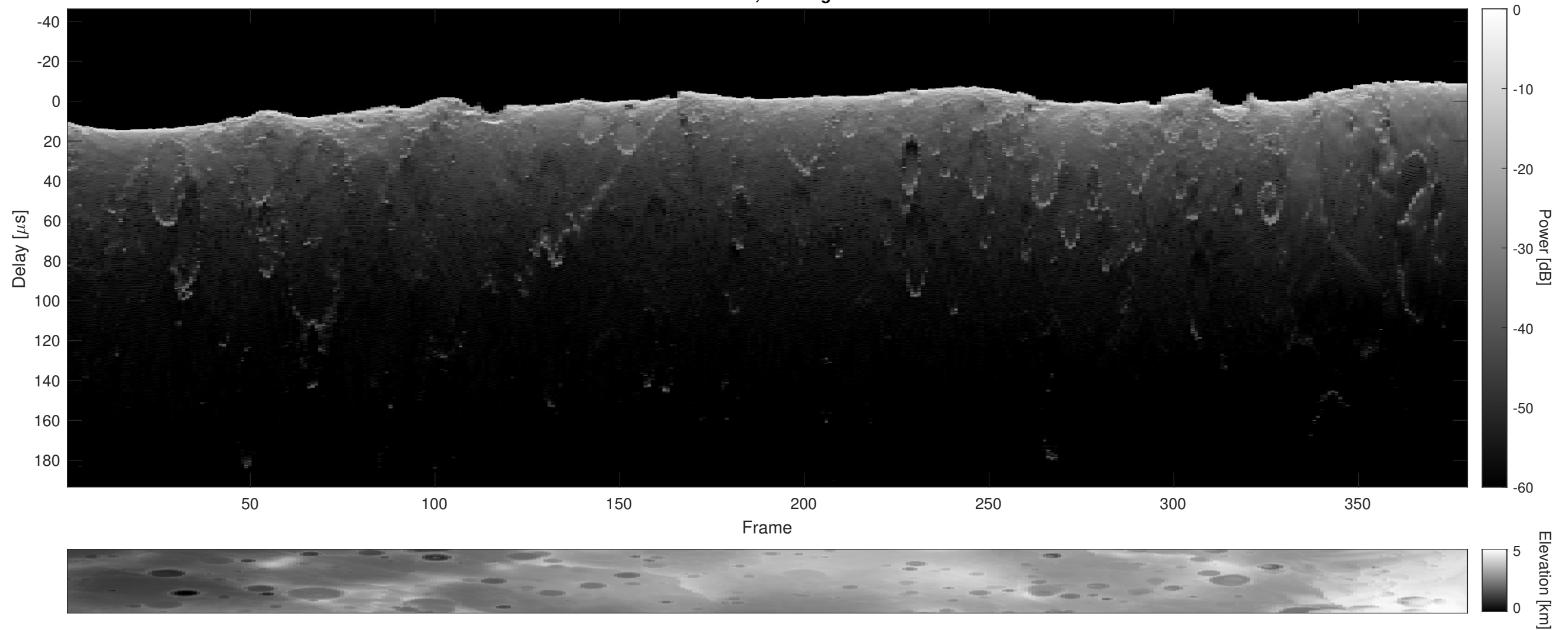
Orbit 2929, Cluttergram
