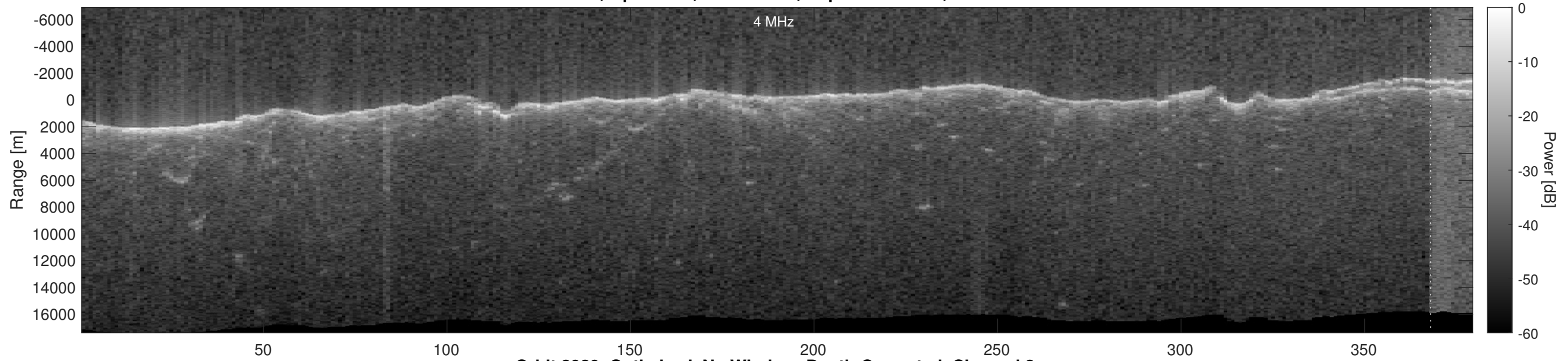
Orbit 2929, Optimized, No Window, Depth-Corrected, Channel 2
