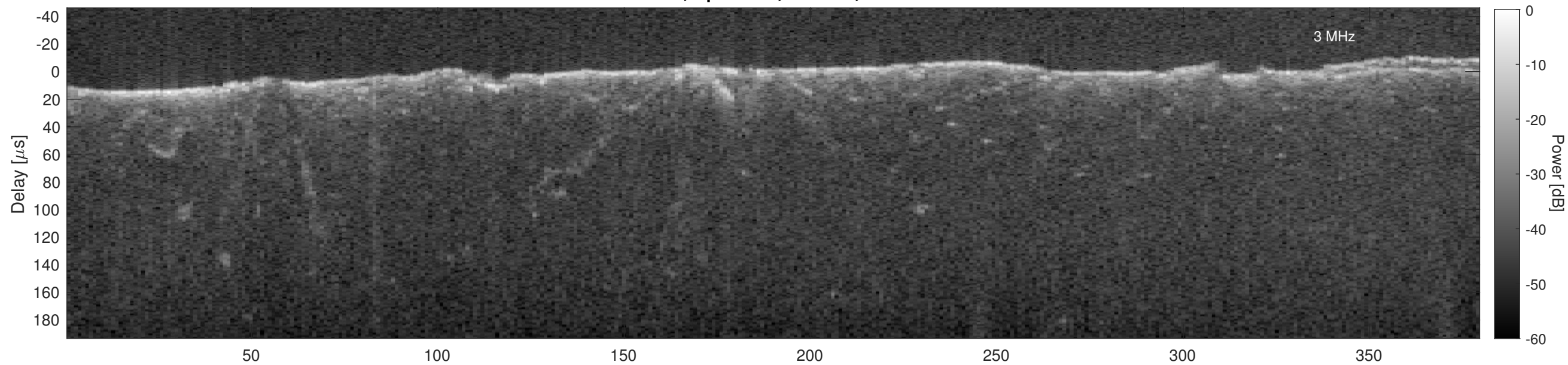
Orbit 2929, Cluttergram
