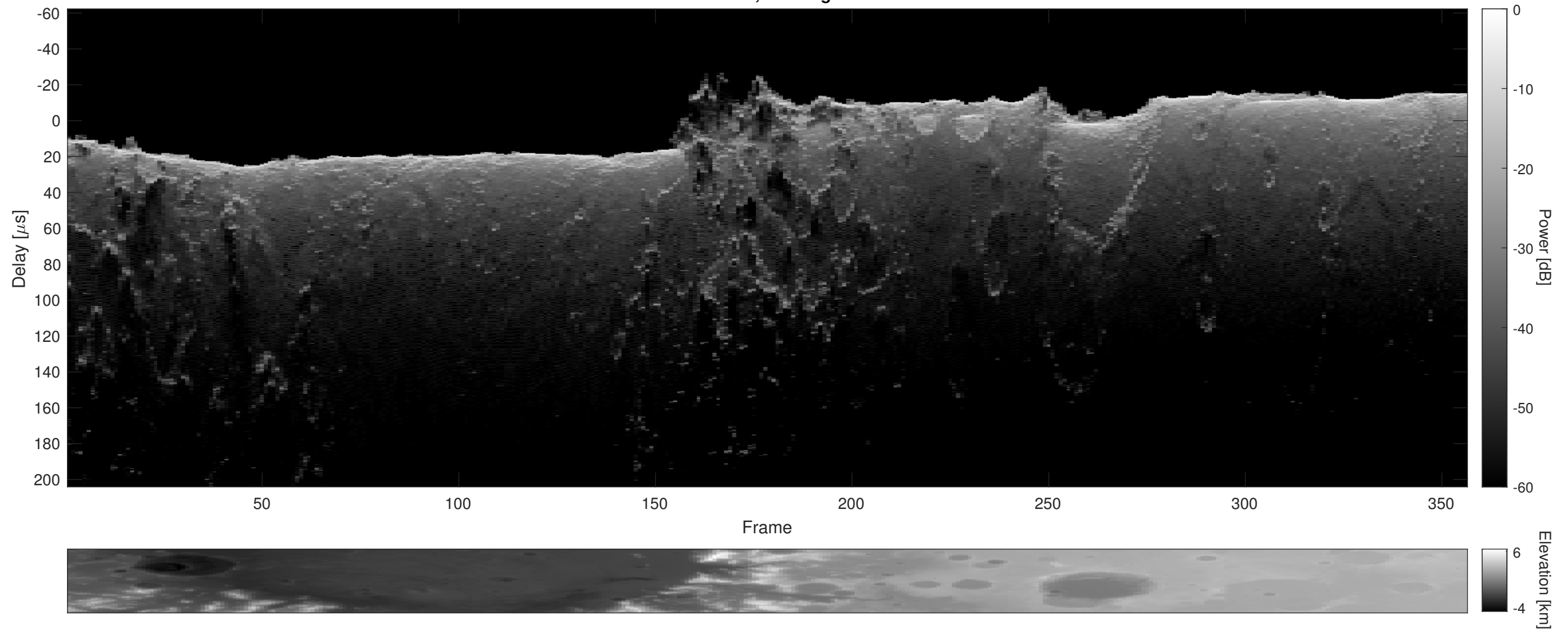
Orbit 2931, Cluttergram
