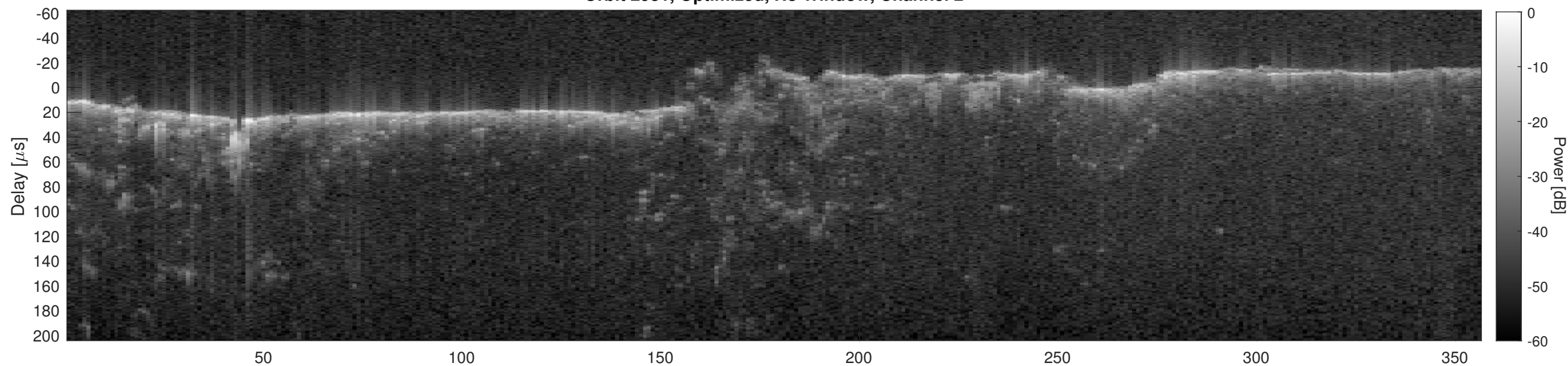
Orbit 2931, Cluttergram
