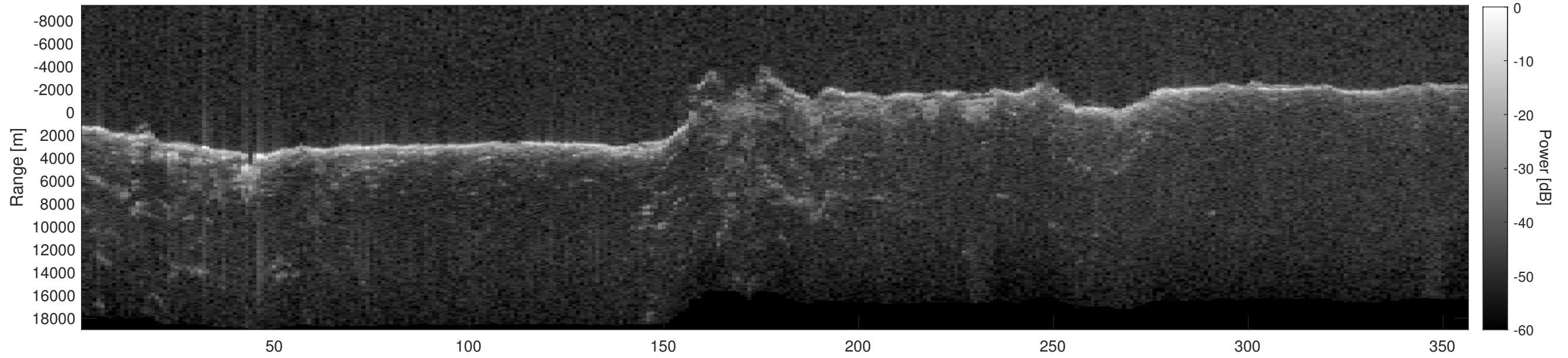
Orbit 2931, Depth-Corrected Cluttergram
