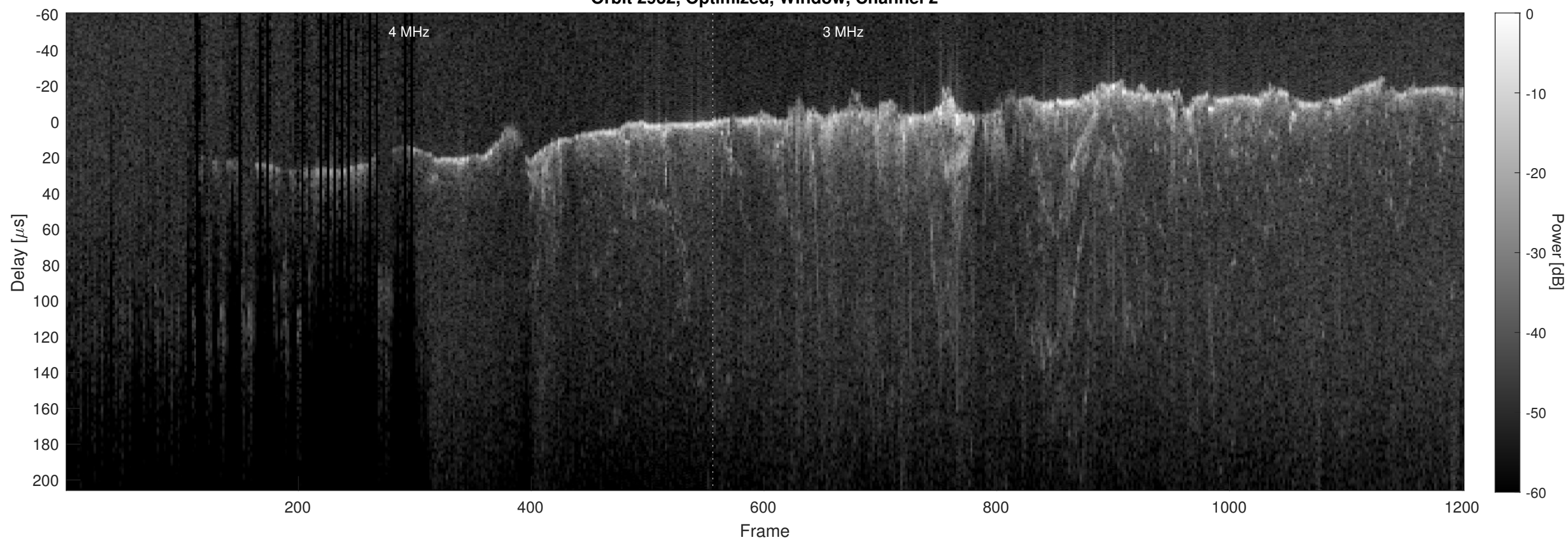
Orbit 2932, Optimized, Window, Channel 2
