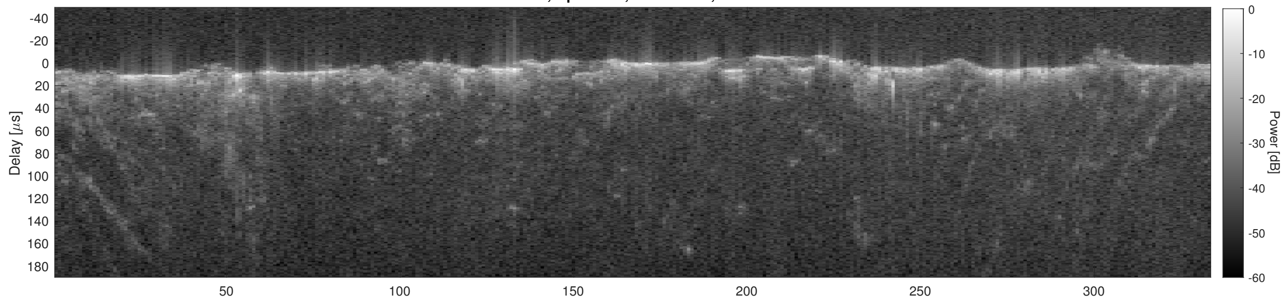
Orbit 2933, Cluttergram
