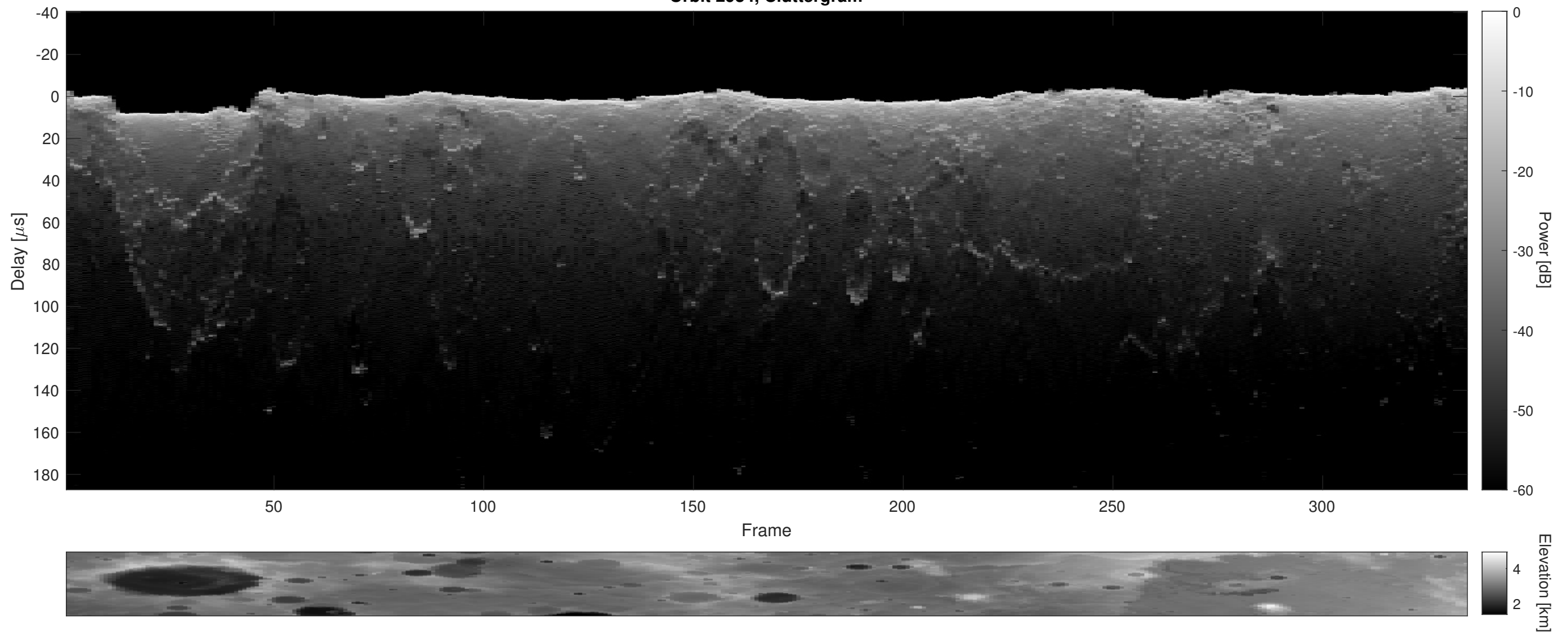
Orbit 2934, Cluttergram
