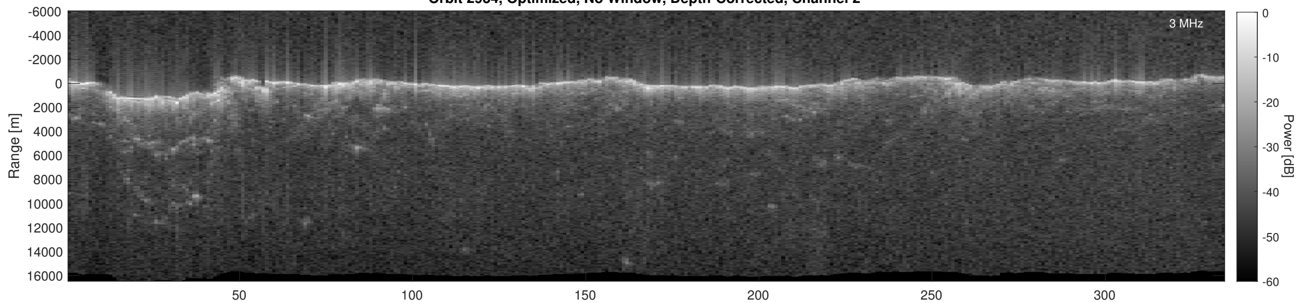
Orbit 2934, Depth-Corrected Cluttergram
