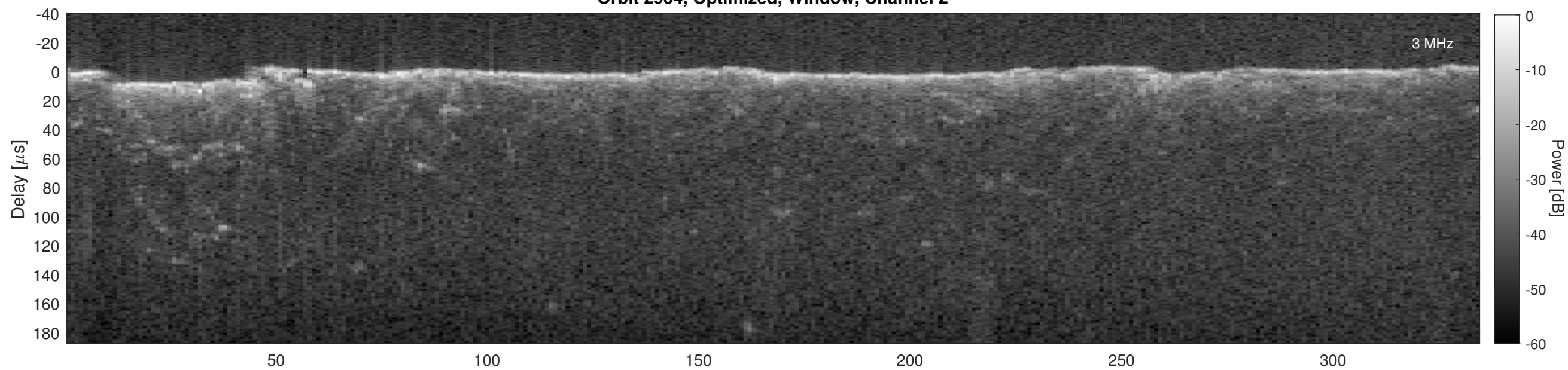
Orbit 2934, Cluttergram
