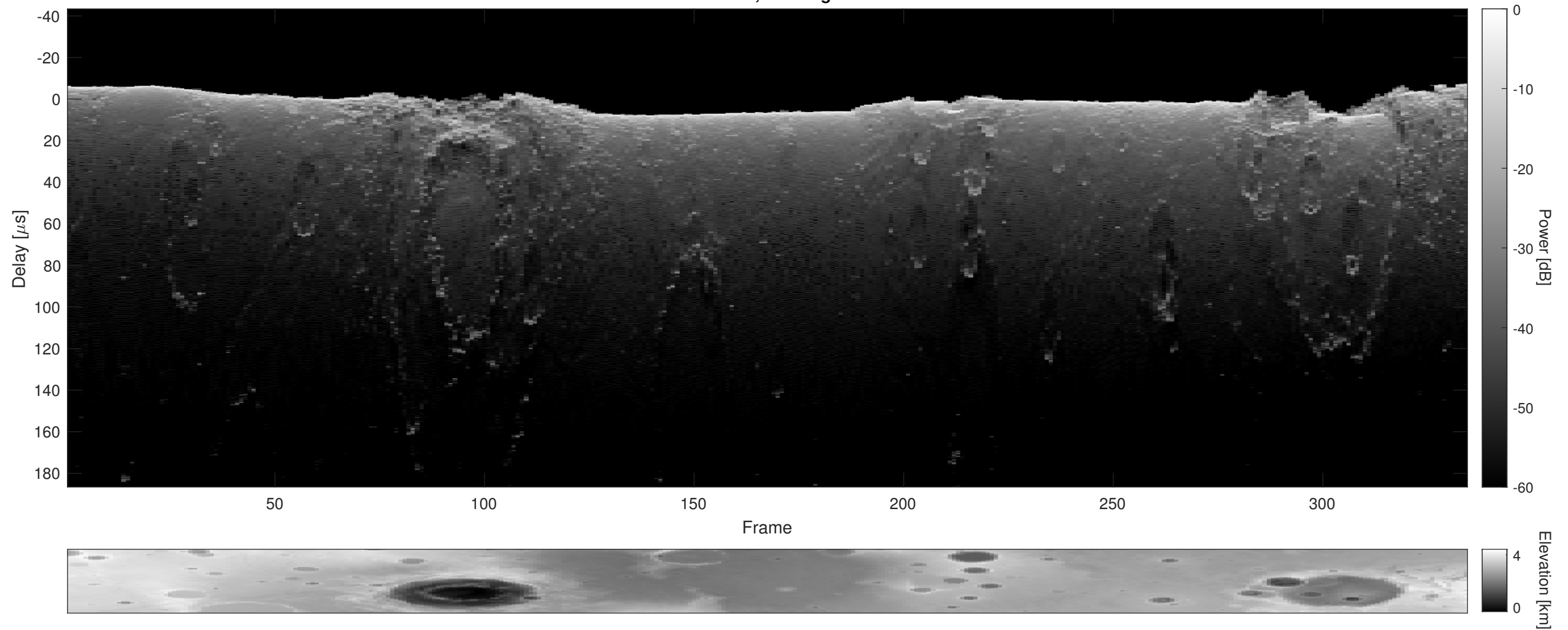
Orbit 2935, Cluttergram
