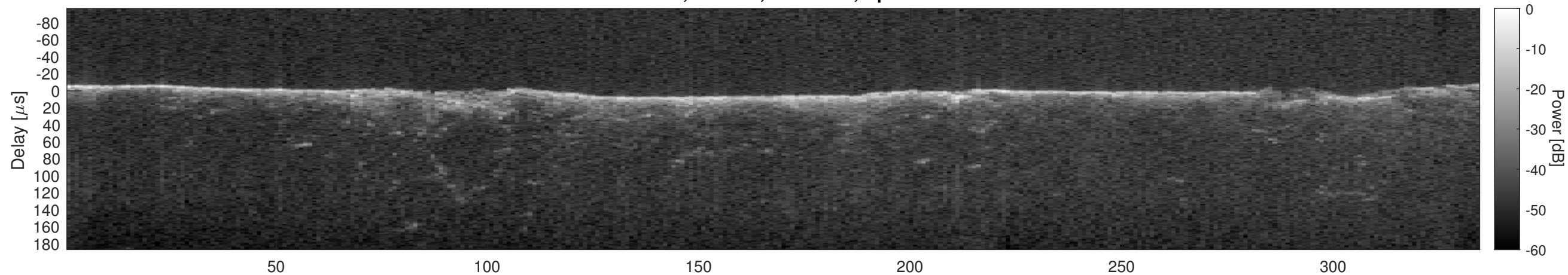
Orbit 2935, Cluttergram
