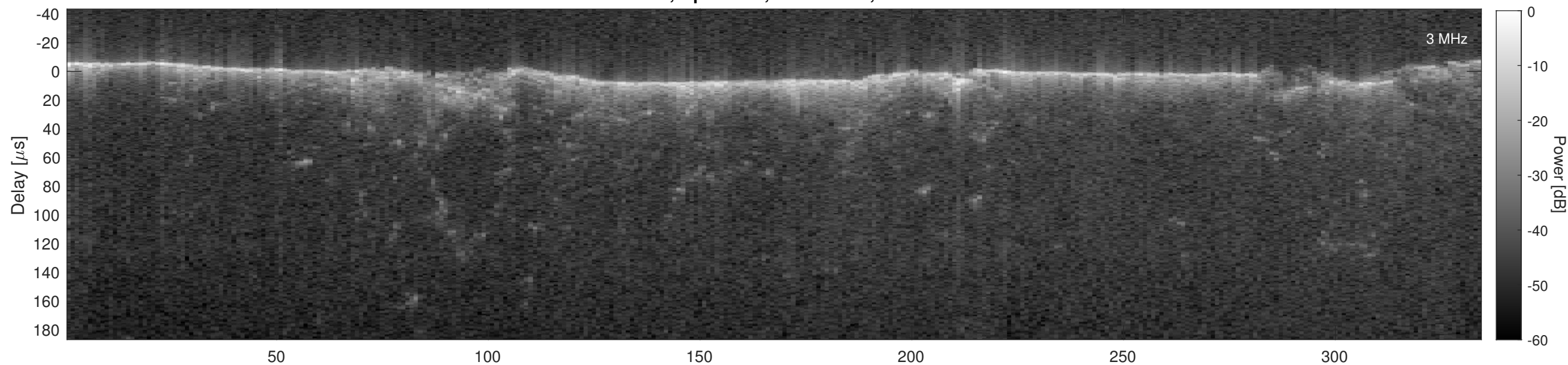
Orbit 2935, Cluttergram
