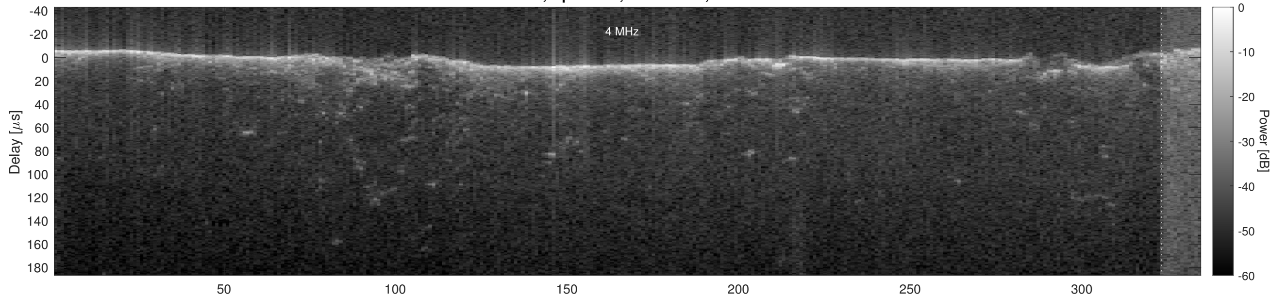
Orbit 2935, Optimized, No Window, Channel 2
