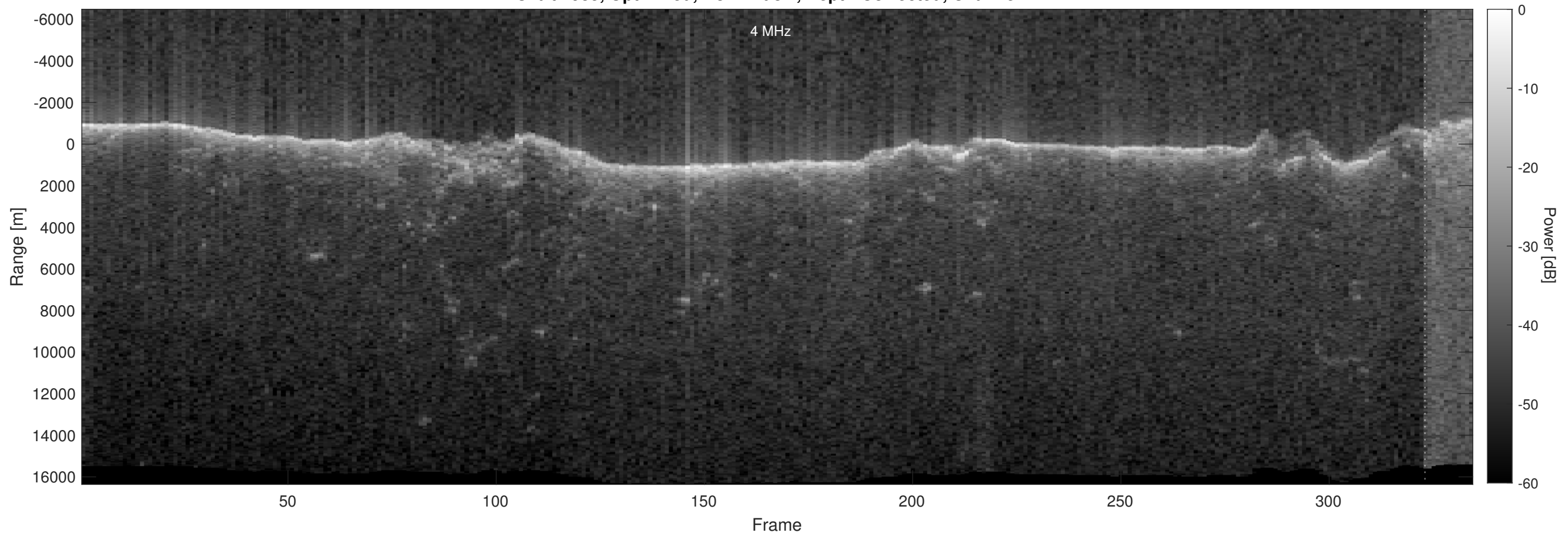
Orbit 2935, Optimized, No Window, Depth-Corrected, Channel 2
