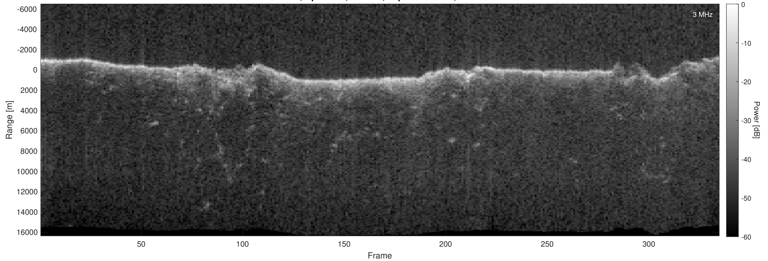
Orbit 2935, Optimized, Window, Depth-Corrected, Channel 2
