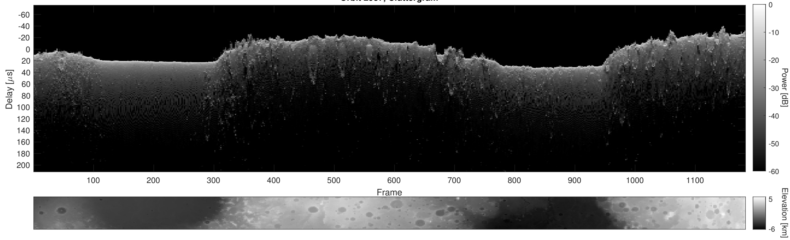
Orbit 2937, Cluttergram
