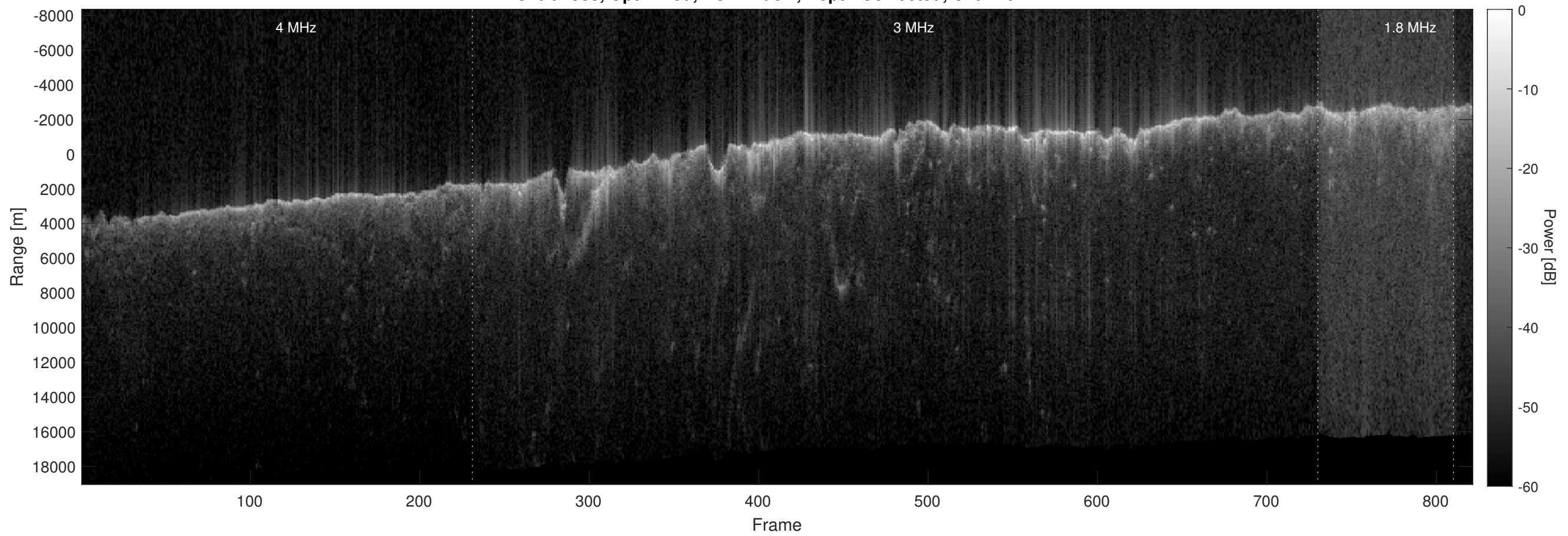
Orbit 2938, Optimized, No Window, Depth-Corrected, Channel 2
