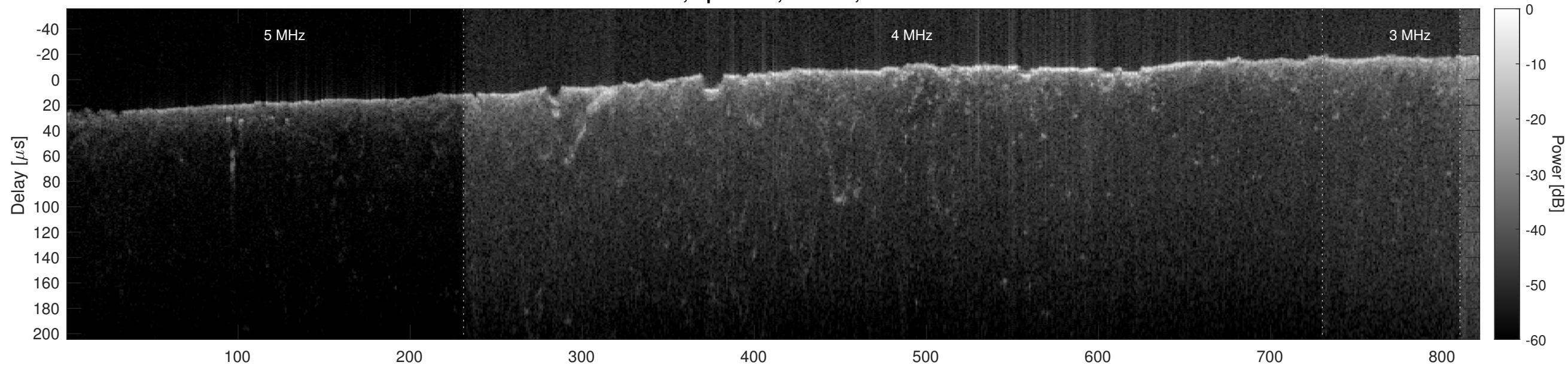
Orbit 2938, Optimized, Window, Channel 2
