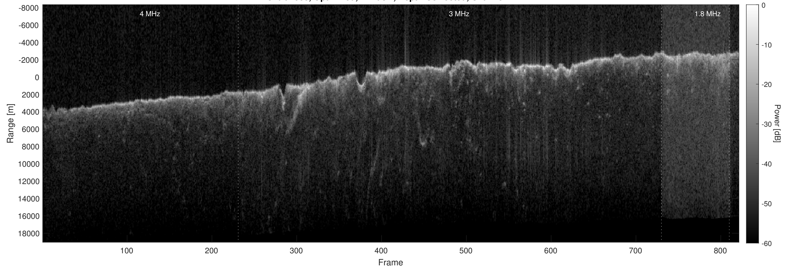
Orbit 2938, Optimized, Window, Depth-Corrected, Channel 2
