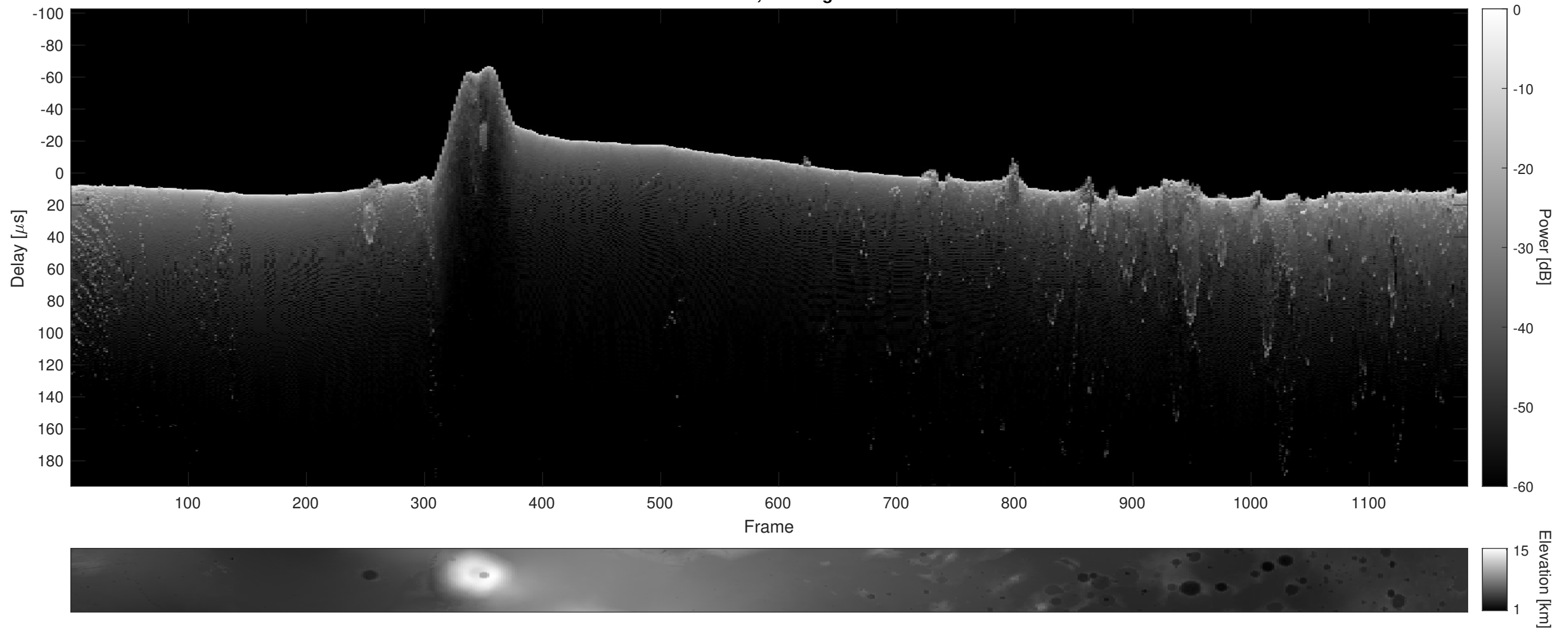
Orbit 2939, Cluttergram
