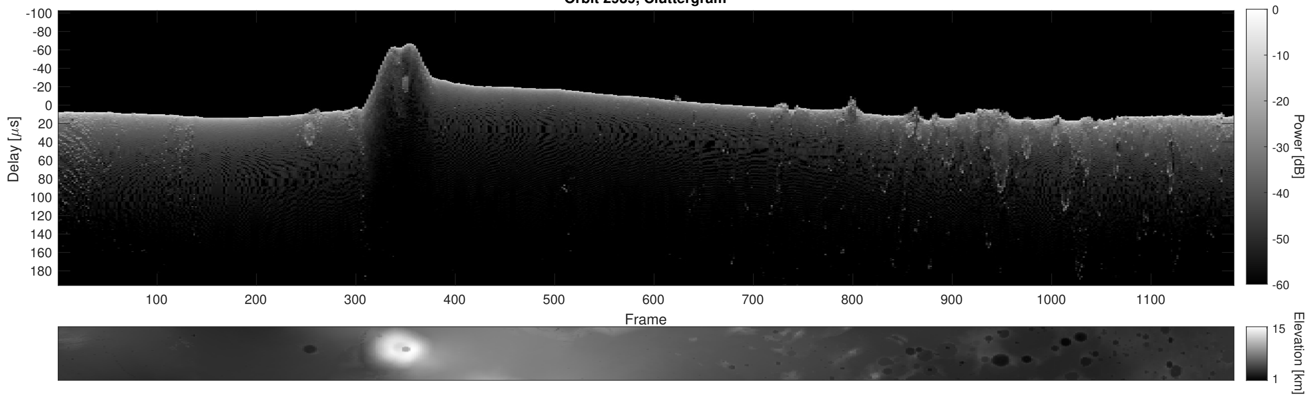
Orbit 2939, Cluttergram
