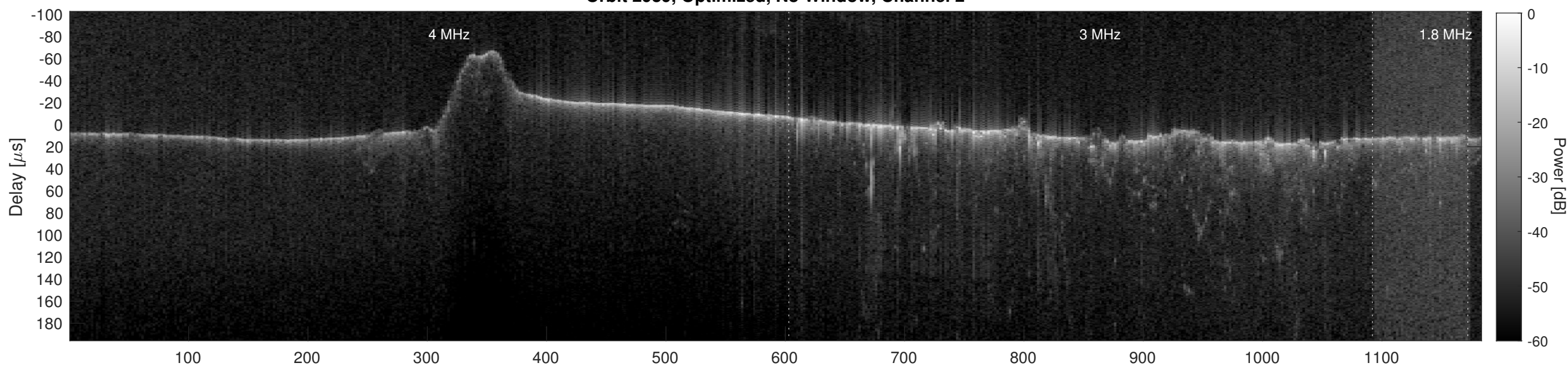
Orbit 2939, Cluttergram
