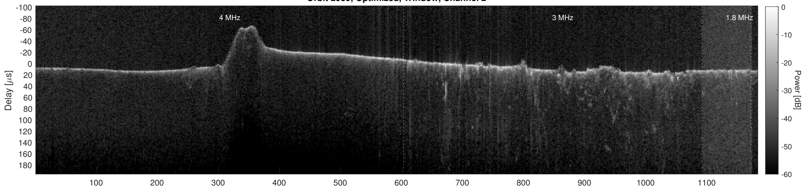
Orbit 2939, Cluttergram
