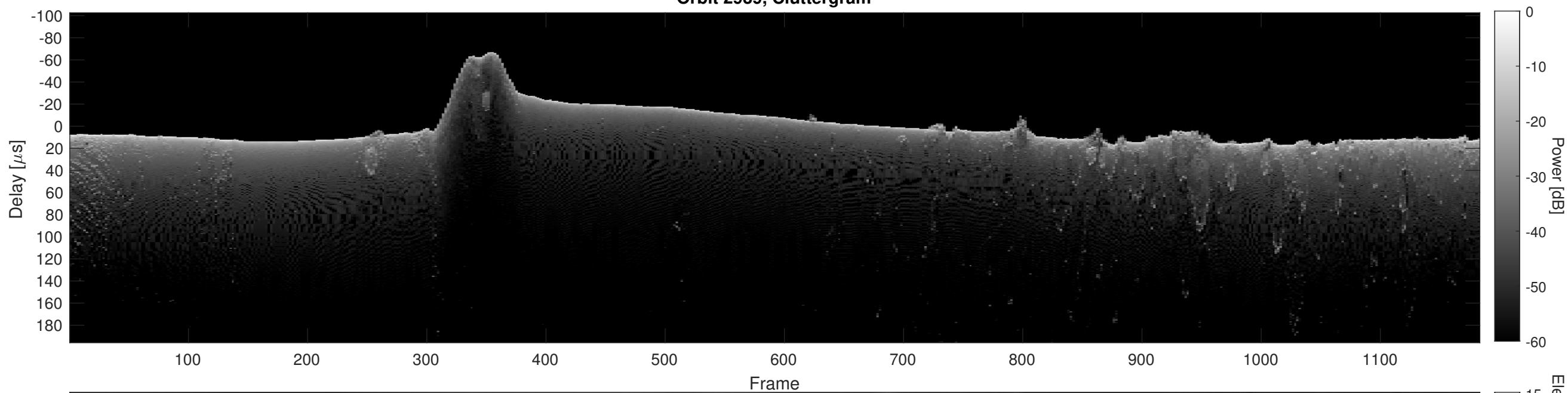
Orbit 2939, Cluttergram
