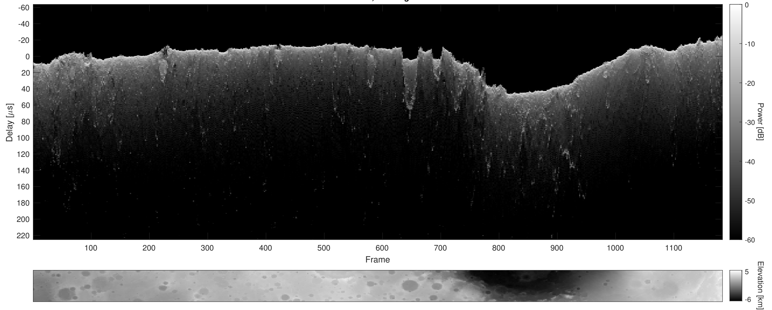
Orbit 2941, Cluttergram
